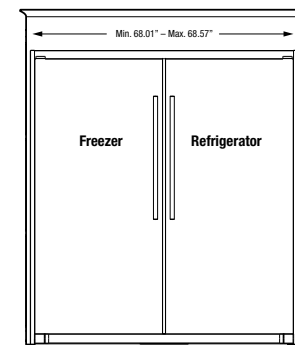
75" Dual Trim kit Flat Design TRMKTEZ2FL75
